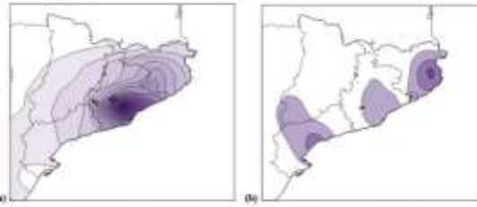
Fig. 7. Contours of tornado occurrence density for the periods 1960–2009 (a) and 1950–1979 (b). The interval contours are 1 case 0.5° x 0.5° latitude longitude.
